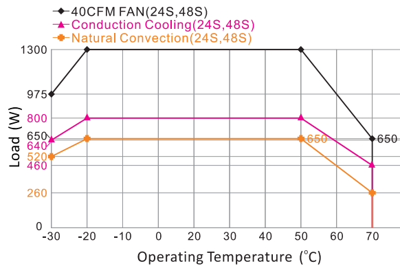
Derating Output Load versus Operating Temperature VPF1300E-24S,48S at 198-264Vin
