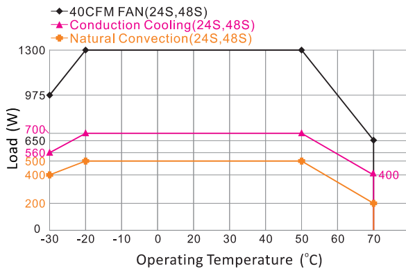
Derating Output Load versus Operating Temperature VPF1300E-24S,48S at 115-197Vin
