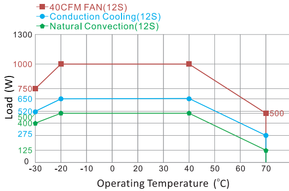
Derating Output Load versus Operating Temperature VPF1300E-12S at 115-197Vin
