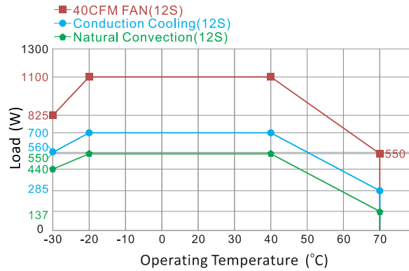
Derating Output Load versus Operating Temperature VPF1300E-12S at 198-264Vin
