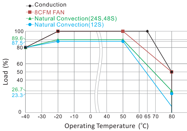
Derating Output Load versus Operating Temperature VPF240U/VP F240E at 100-197Vin
