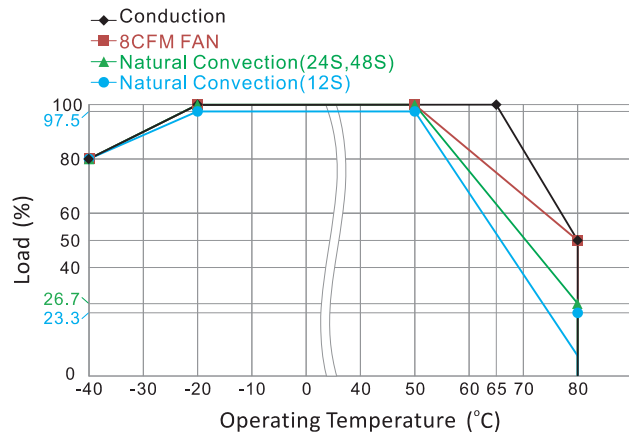
Derating Output Load versus Operating Temperature VPF240U/VP F240E at 198-264Vin
