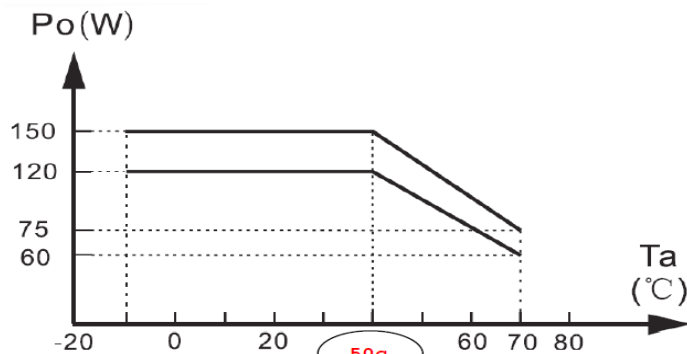
Output Power Vs Ambient Temperature
