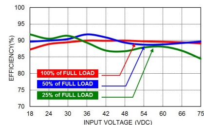
VPQ60-48S24W Efficiency vs. Input Voltage
