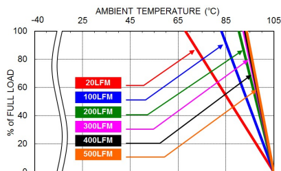
VPQ60-48S24W Derating Curve With Heat-sink
