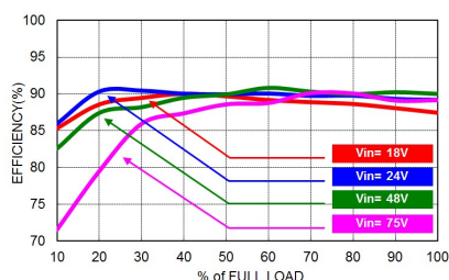
VPQ60-48S24W Efficiency vs. Output Load
