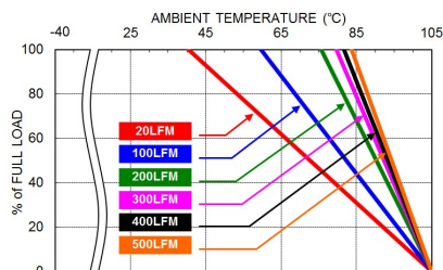
VPQ60-48S24W Derating Curve
