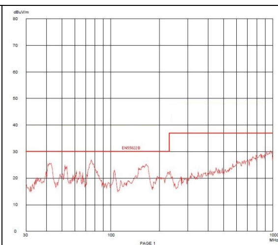
Typical Radiated emissions
