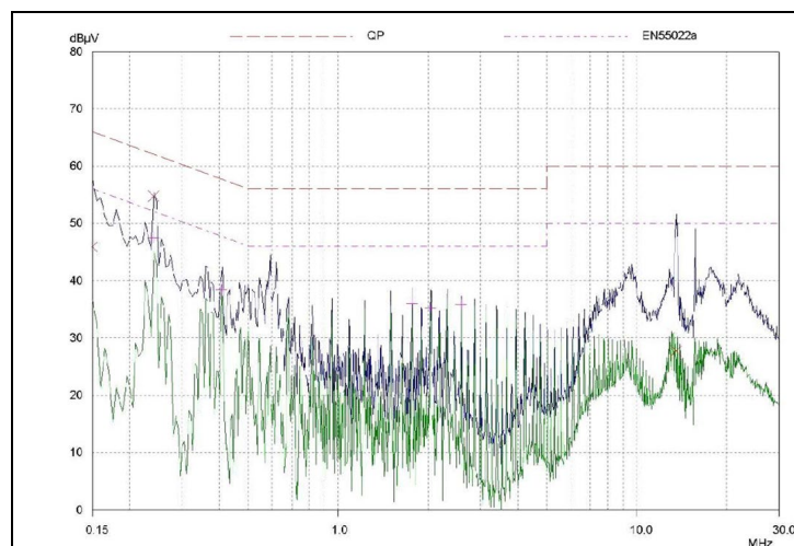
Typical Conducted emissions
