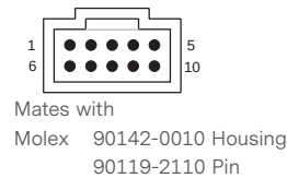
Figure 2. Connector J1
