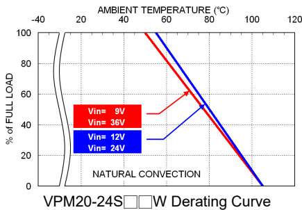
VPM20-24S□□W Derating Curve
