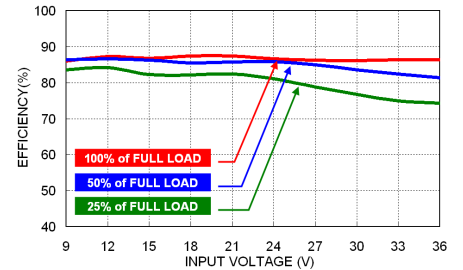
VPM20-24S05W Efficiency vs. Input Voltage
