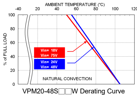
VPM20-48S□□W Derating Curve
