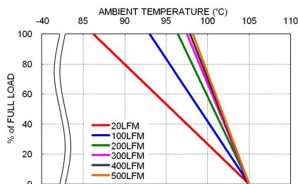
VPP06-48S05WA Derating Curve
