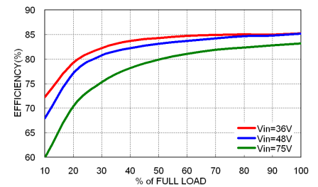
VPP06-48S05WA Efficiency vs. Output Load
