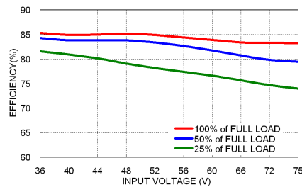
VPP06-48S05WA Efficiency vs. Input Voltage
