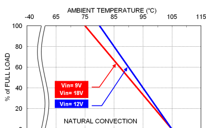
VPS(H)04-12□□□ Derating Curve
