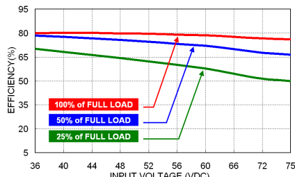
VPS(H)04-48S05 Efficiency vs. Input Voltage
