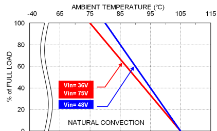
VPS(H)04-48□□□ Derating Curve
