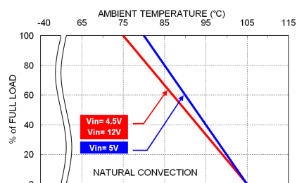
VPS(H)04-05□□□ Derating Curve
