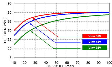
VPS(H)04-48S05 Efficiency vs. Output Current
