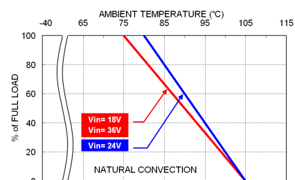
VPS(H)04-24□□□ Derating Curve
