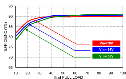
VPD15-24S05 Efficiency vs. Output Load
