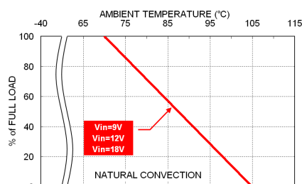
VPD15-12 Derating Curve
