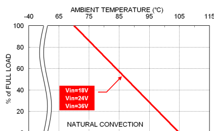
VPD15-24 Derating Curve
