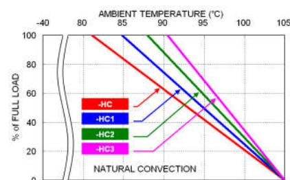
VPD15-24S05 Derating Curve With Heat-sink
