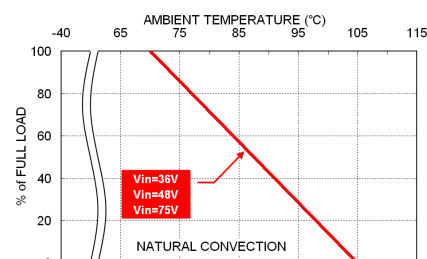
VPD15-48 Derating Curve
