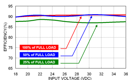
VPD15-24S05 Efficiency vs. Input Voltage
