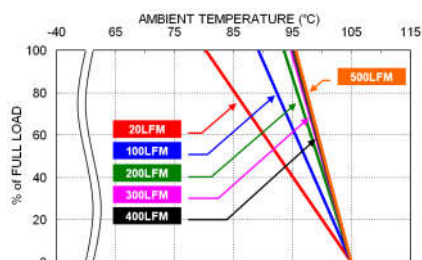
VPD10-48S3P3W Derating Curve
