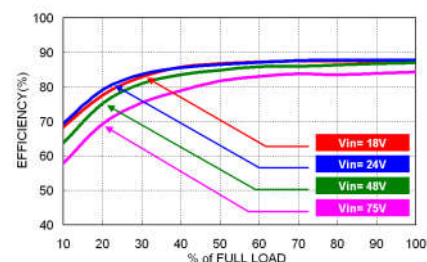
VPD10-48S3P3W Efficiency vs. Output Load
