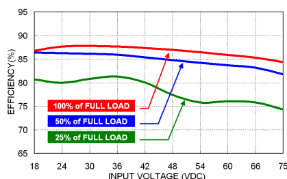
VPD10-48S3P3W Efficiency vs. Input Voltage
