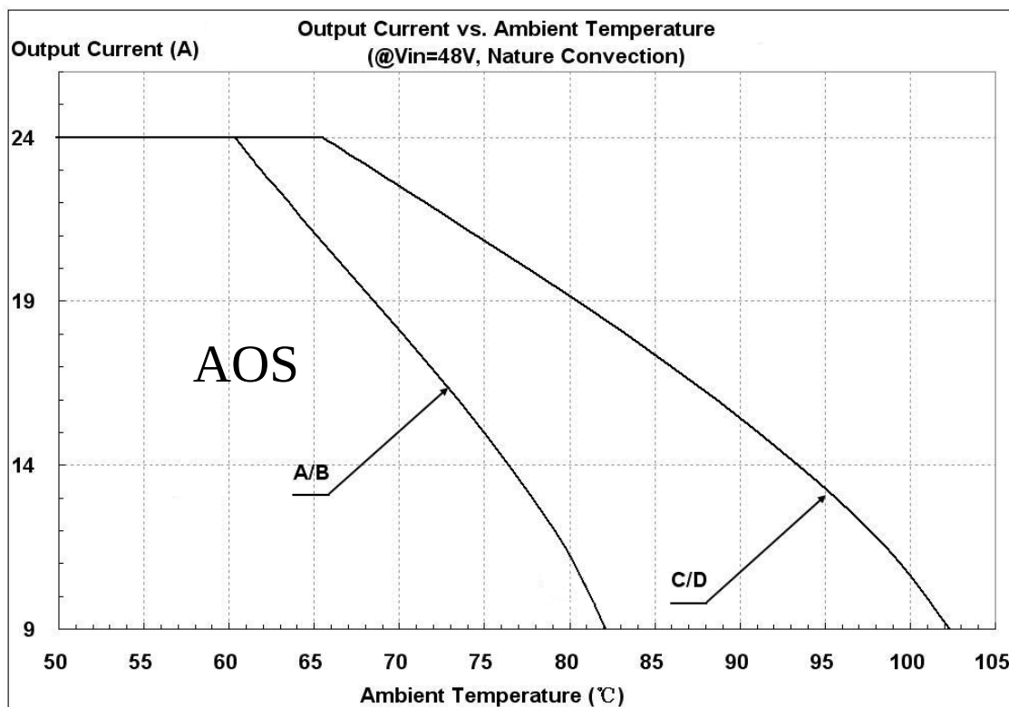
Figure 17: Output Current vs. ambient temperature @Vin=48V
