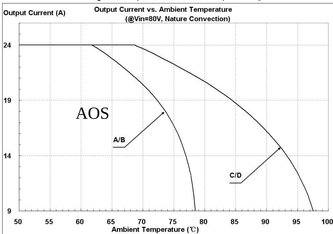
Figure 19: Output Current vs. ambient temperature @Vin=80V
