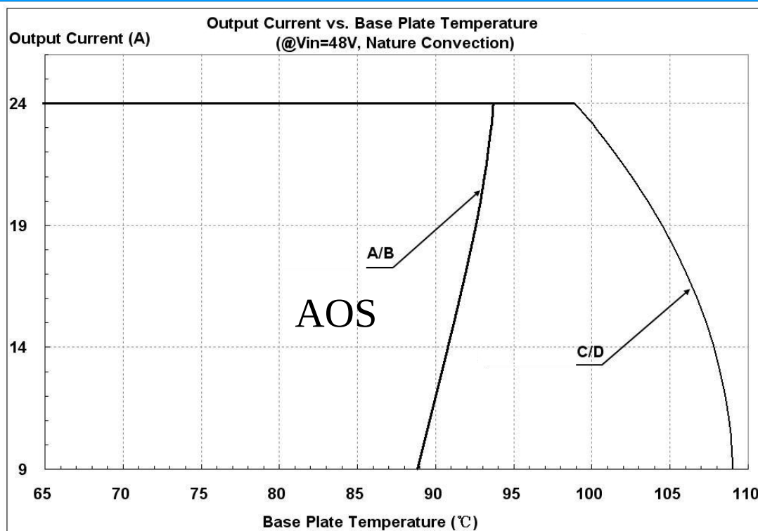
Figure 21: Output Current vs. base plate temperature @Vin=48V
