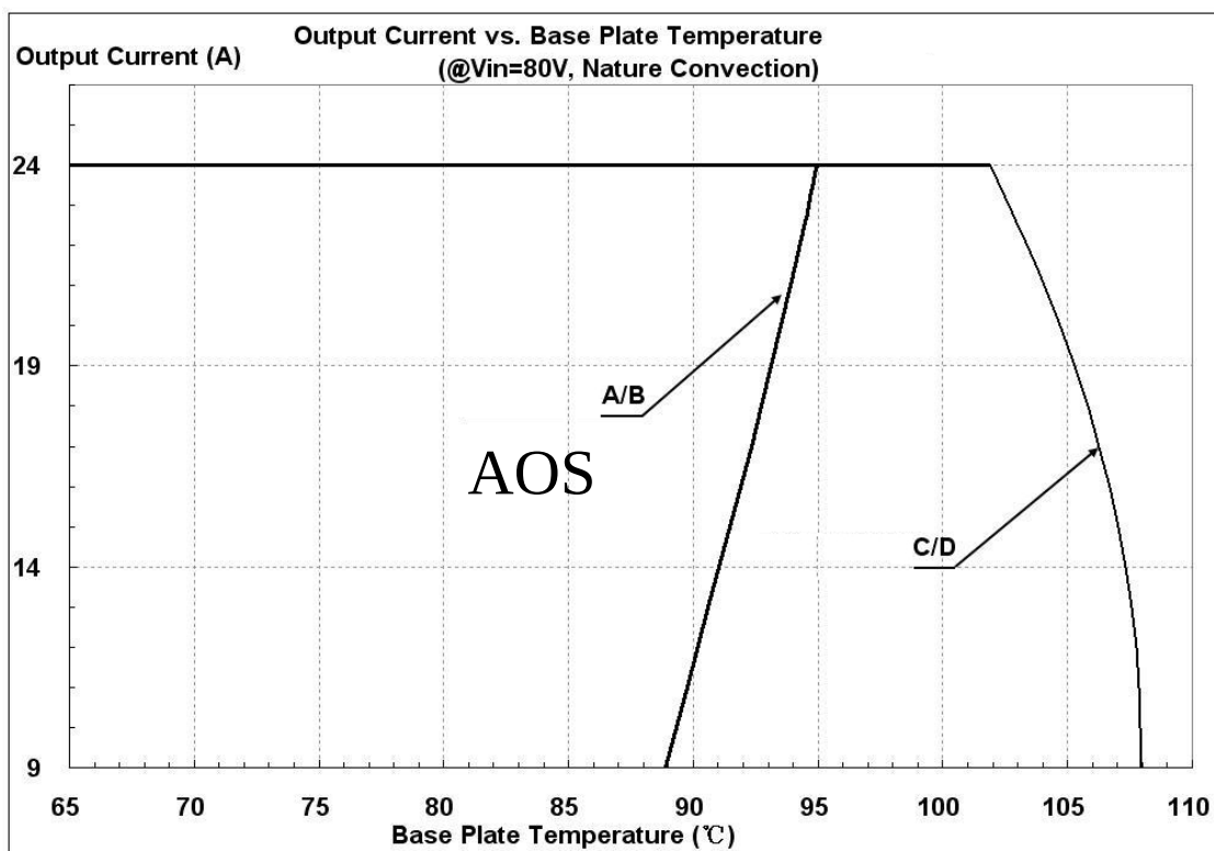
Figure 23: Output Current vs. base plate temperature @Vin=80V
