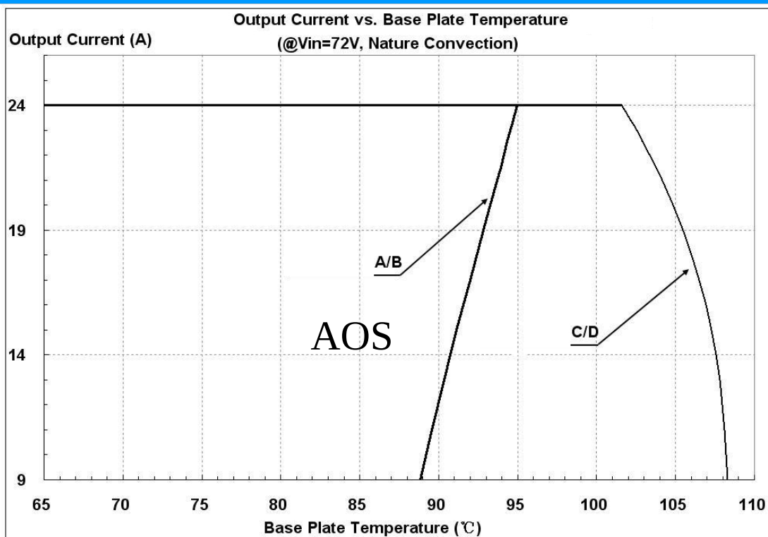
Figure 22: Output Current vs. base plate temperature @Vin=72V
