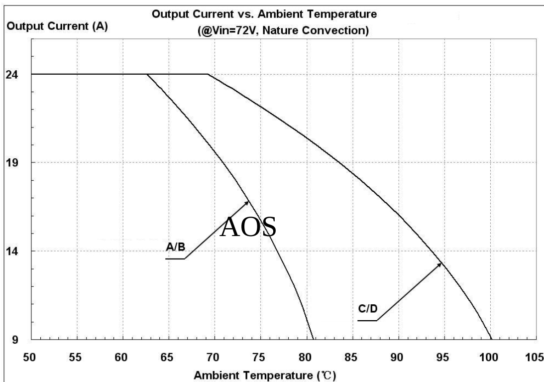
Figure 18: Output Current vs. ambient temperature @Vin=72V
