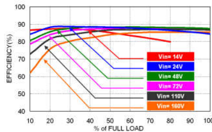
VPE100-72S05U Efficiency vs. Output Load
