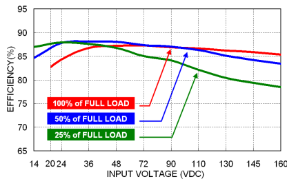
VPE100-72S05U Efficiency vs. Input Voltage
