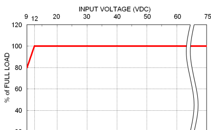
Derating Curve vs. Input Voltage VPE100-36S U
