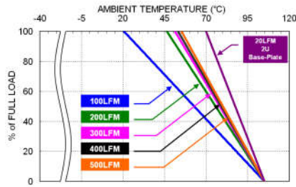
VPE100-72S05U Derating Curve (See Thermal Considerations)
