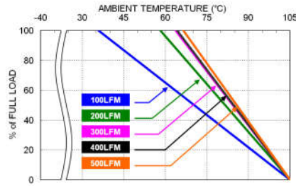
VPE100-72S05U Derating Curve With 0.24" Height Heat-sink (See Thermal Considerations)
