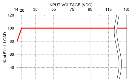
Derating Curve vs. Input Voltage VPE100-72S U
