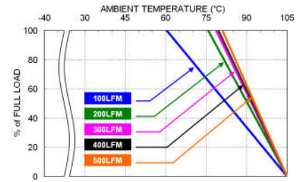
VPE100-72S05U Derating Curve With 0.5" Height Heat-sink (See Thermal Considerations)
