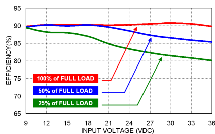
VPD15-24S05W Efficiency vs. Input Voltage
