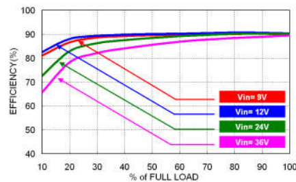
VPD15-24S05W Efficiency vs. Output Load
