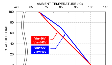
VPD15-110 0.5W Derating Curve
