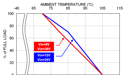
VPD15-24 0.5W Derating Curve
