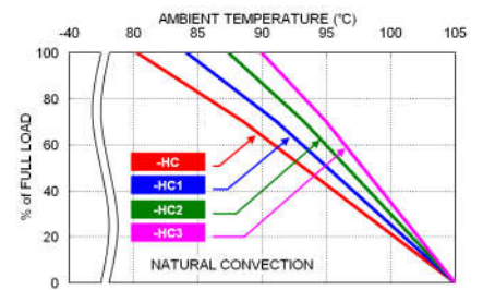
VPD15-24S05W Derating Curve With Heat-sink
