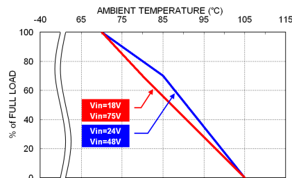
VPD15-48 0.5W Derating Curve
