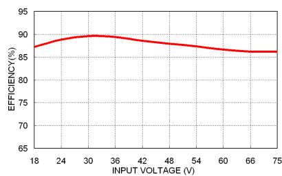
VPC08-48S05W Efficiency vs. Input Voltage
