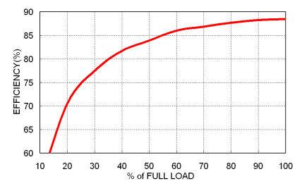
VPC08-48S05W Efficiency vs. Output Load
