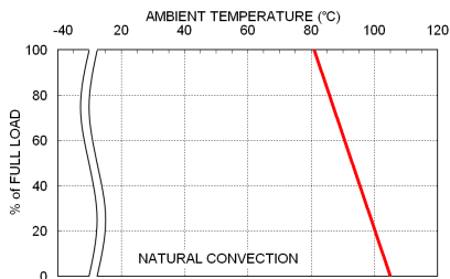
VPC08-48S05W Derating Curve
