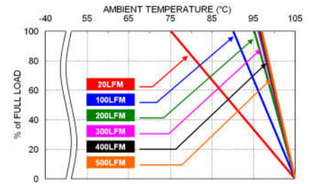
VPE40-72S05U Derating Curve With 0.5" Height Heat-sink (See Thermal Considerations)
