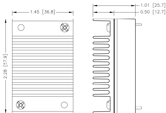
VPE40-□□S□□U – HS1 7G-0030B-F
