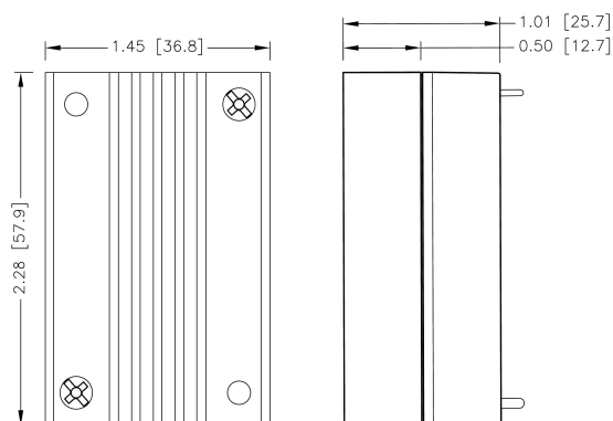
VPE40-□□S□□U – HS3 7G-0032B-F
