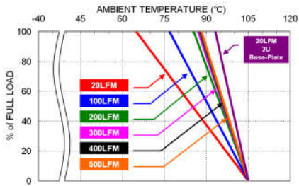
VPE40-72S05U Derating Curve (See Thermal Considerations)
