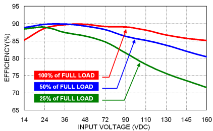
VPE40-72S05U Efficiency vs. Input Voltage
