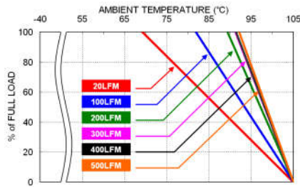
VPE40-72S05U Derating Curve With 0.24" Height Heat-sink (See Thermal Considerations)
