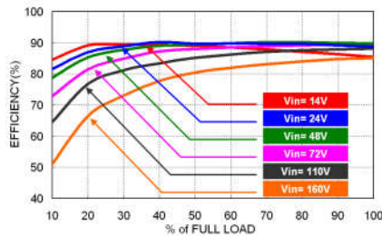
VPE40-72S05U Efficiency vs. Output Load
