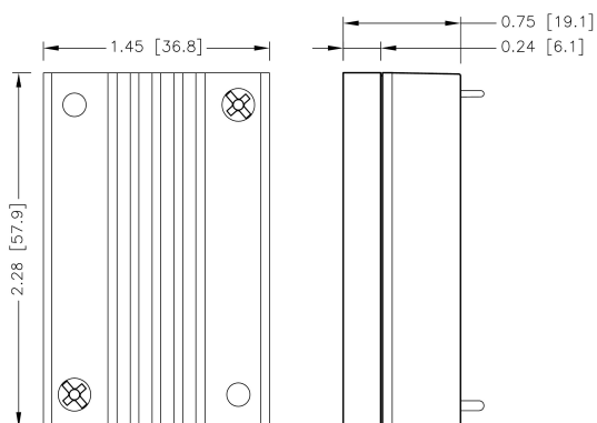
VPE40-□□S□□U – HS2 7G-0031B-F
