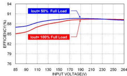
VPAD30US24B Efficiency vs. Input Voltage
