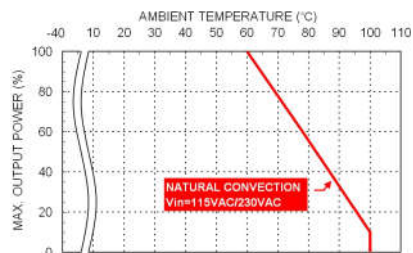
Derating Curve vs. Ambient Temperature VPAD30USxxB xx=3P3/05/7P5/09/121/151/18 Connector Option : (-M / -T / -D)
