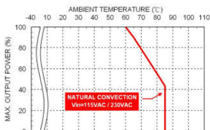
Derating Curve vs. Ambient Temperature VPAD30USxxB xx=3P3/05/7P5/09/121/151/18 Connector Option : (□: JST)
