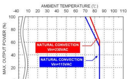
Derating Curve vs. Ambient Temperature VPAD30USxxB xx=12/15/24/28/36/48/53 Connector Option : (□: JST)
