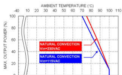
Derating Curve vs. Ambient Temperature VPAD30USxxB xx=12/15/24/28/36/48/53 Connector Option : (-M / -T / -D)
