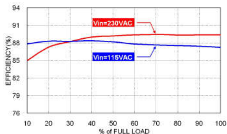
VPAD30US24B Efficiency vs. Output Load
