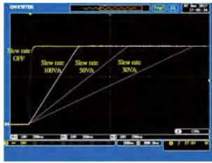
Adjustable Voltage Slew Rate
