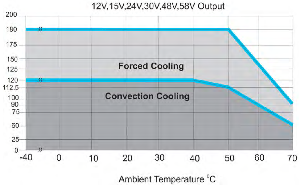
Derating Curve
